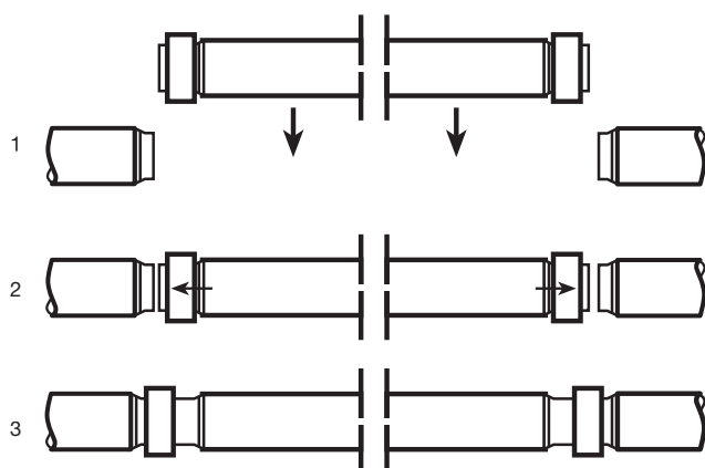
Figure 3-1-2: Closure piece
